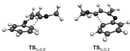
Figure 2. Geometries of the ring-closing transition states \text{TS}_{\text{C-C,E}} and \text{TS}_{\text{C-C,Z}} .
