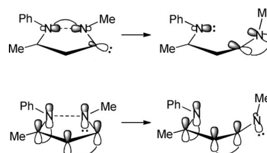
Figure 3. Reorganization of \sigma (top) and \pi (bottom) electrons of A upon ring opening. Curved lines and dots indicate bonding and nonbonding pairs according to one of the high-weight resonance forms.
