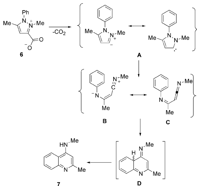
Scheme 2. Rearrangement of pyrazolium-3-carboxylates to 4-aminoquinolines via N-heterocyclic carbenes of pyrazole.
