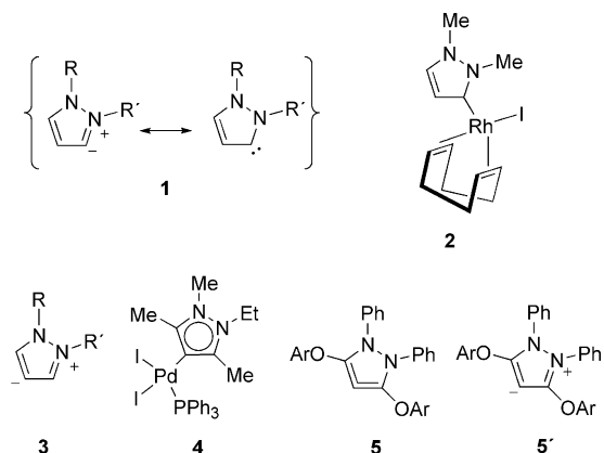
Scheme 1. N-Heterocyclic carbenes of pyrazole.
