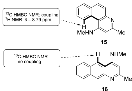
Scheme 6. Diagnostic NMR results.
