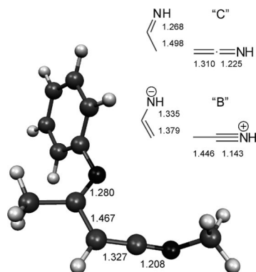
Figure 4. Computed geometry of intermediate E -C. Calculated bond lengths (Å) of some model compounds formally corresponding to parts of resonance structures B and C are also given for comparison. Similar results were obtained for Z -C.
