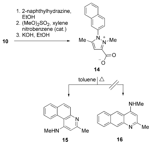
Scheme 5. Regioselective rearrangement to benzo[ f ]quinolin-1-amine.
