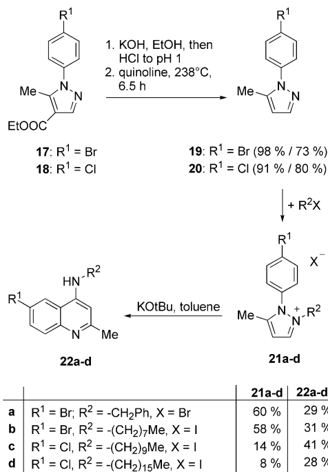
Scheme 7. Rearrangements starting from pyrazolium salts.
