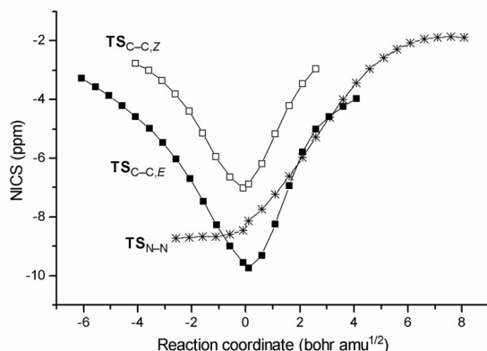
Figure 5. NICS values as a function of the intrinsic reaction coordinate for ring-opening via TS_{N-N} and ring-closing reactions via TS_{C-C,E} and TS_{C-C,Z} .
