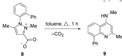
Scheme 3. Synthesis of 4-aminoquinolines.
