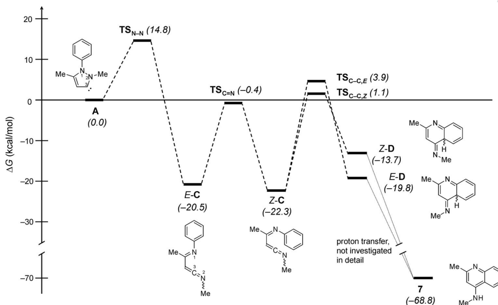
Figure 1. Calculated solvent-phase Gibbs free energy profile for the conversion of A into 7 . Atom numbering used in text is indicated.
